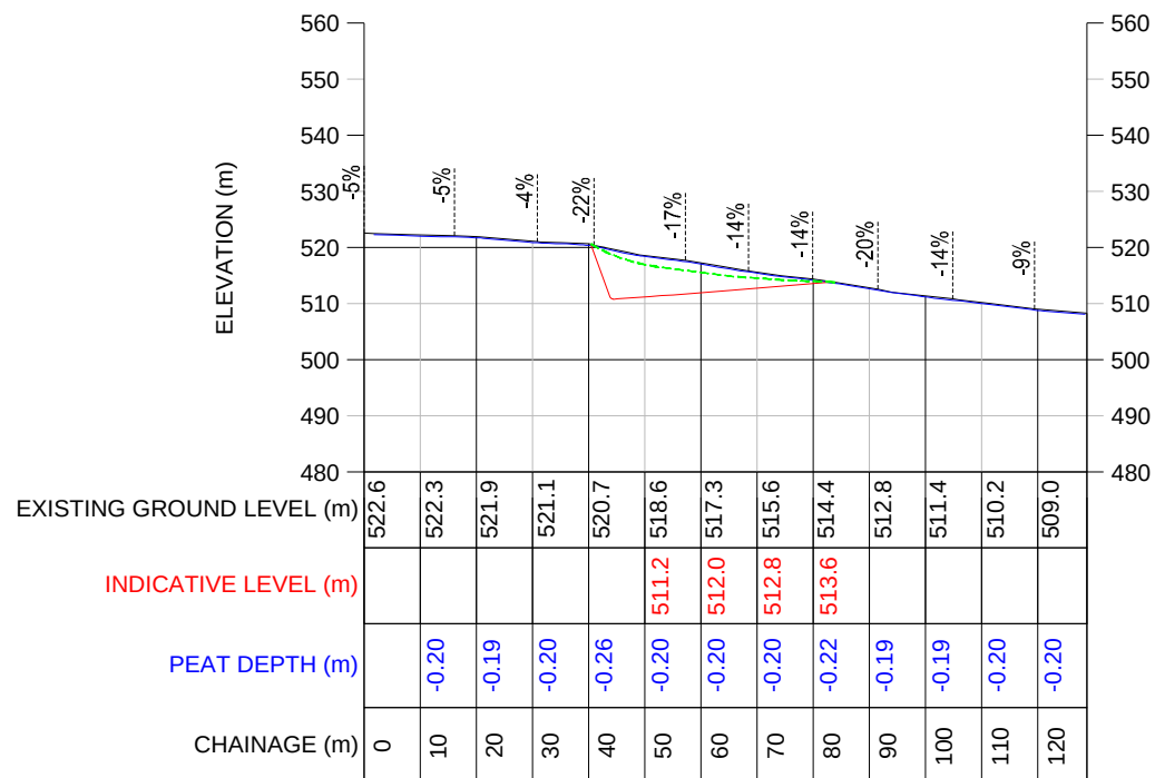
BORROW PIT 1 (BP1)
