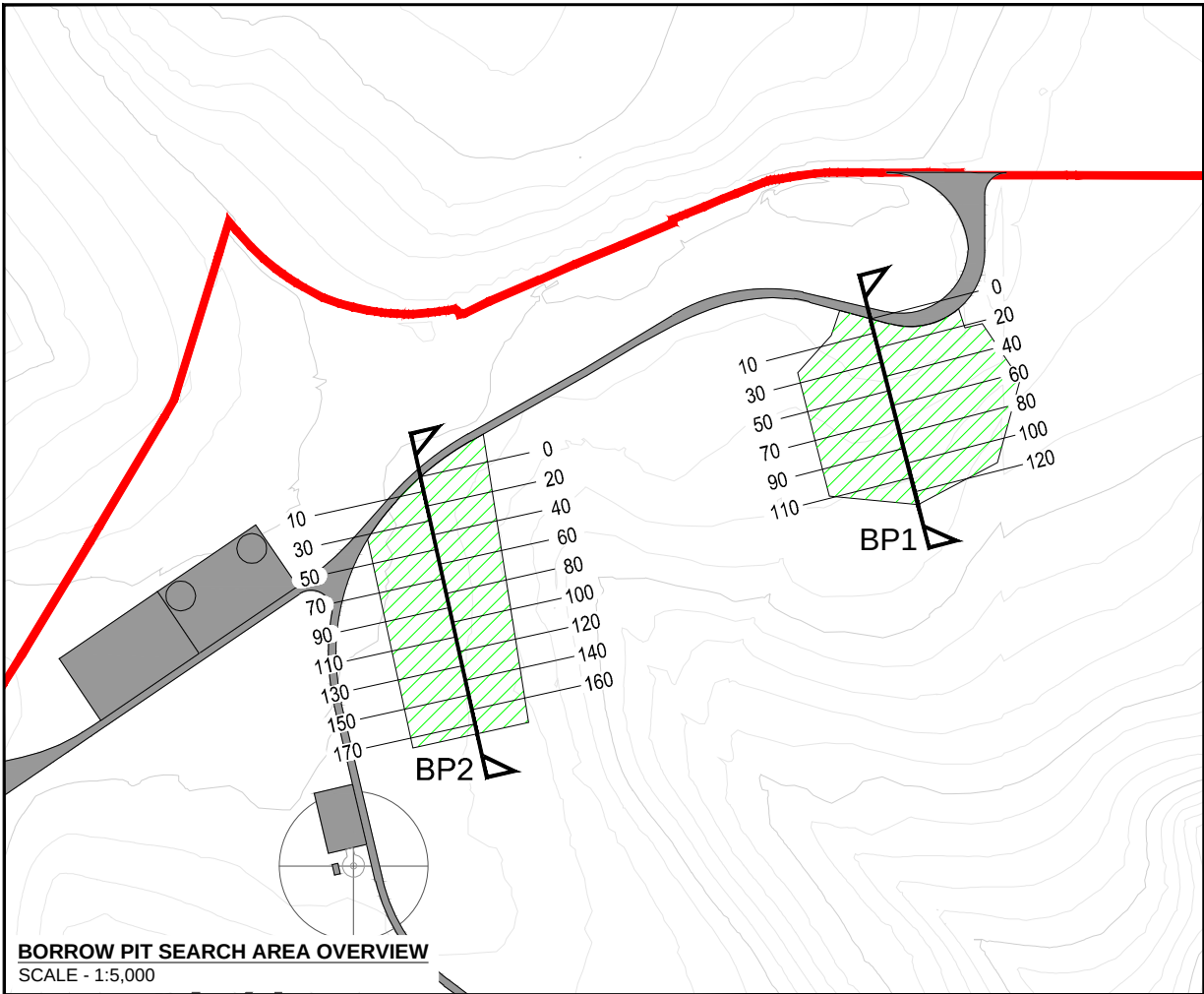
FIGURE 3.11 INDICATIVE BORROW PIT DETAILS
